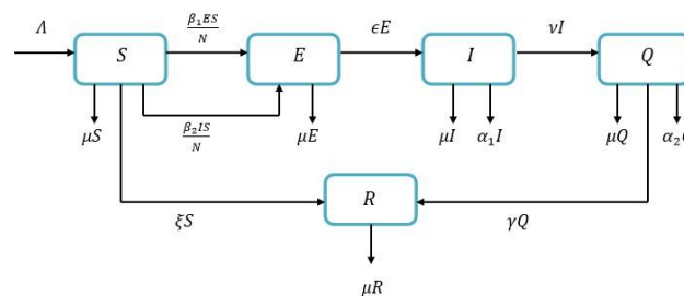
Fig. 1. Schematic diagram for the EVD model.
