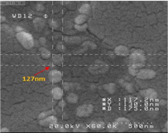
Fig 1. The extracted OMVs from clinical V. cholerae , examined by electron microscopy, contained nano-spheric materials with sizes ranging from 20 to 300 nm.
